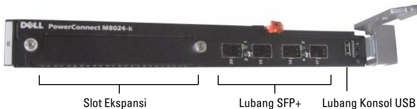
Gambar 1-1. PowerConnect M8024-k Panel Depan
